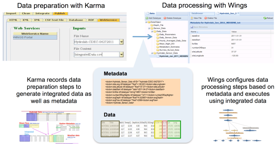
Figure 1. Overview of creation and use of metadata as the data is processed throughout our provenance-aware system.
