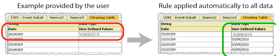
Figure 2. Normalizing the date format: the user provides one example, and the system learns a rule and applies it automatically to the entire dataset.
