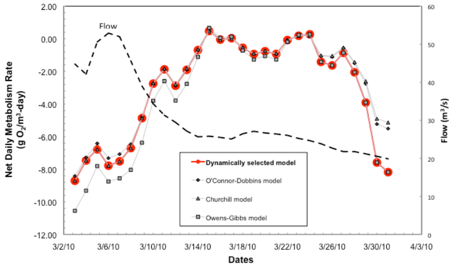
Figure 6. Results from the workflow with reaeration correction by three different models, each optimal at different flow conditions (smaller symbols). The workflow system automatically selects the models (larger red circles) based on flow conditions.
