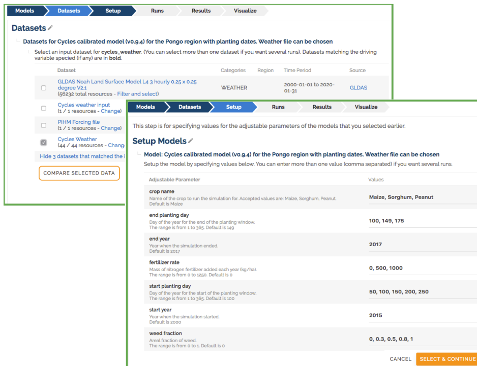
Figure 14: MINT User Interface: Selecting model inputs, both datasets and parameters.
