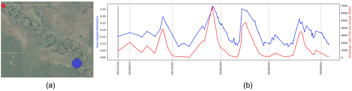
Figure 8: An illustrative example of the potential of satellite imagery analysis to provide calibration data for hydrological models. (a) Study region: St. Johns river near Christmas, Florida. The red star on the image shows the location of the USGS gage station (ID:02232500). The blue circle shows the river segment (~8kms away from the gage station) analyzed using machine learning and satellite imagery from Sentinel 2 between 2015 and 2020. (b) Estimated river segment surface area (in blue) and daily discharge measured from the gage station (in red).
