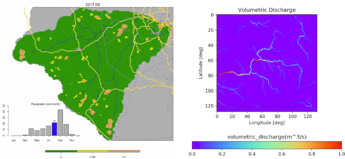
Figure 17: Models of flooding in South Sudan and Ethiopia.
