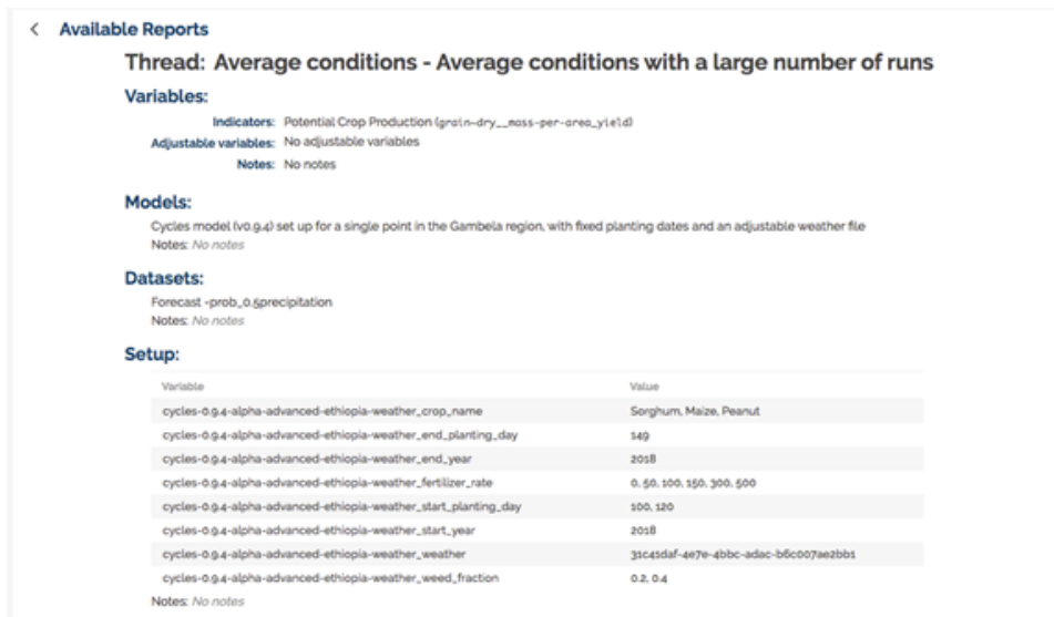
Figure 16: Showing Provenance of Model Results.
