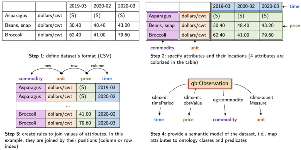
Figure 3: Steps for building a D-REPR model for an agricultural price dataset.
