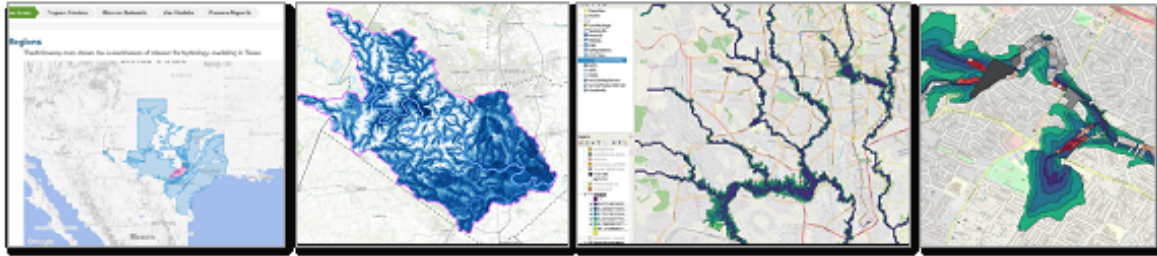
Figure 18: Models of flood vulnerability in central Texas.
