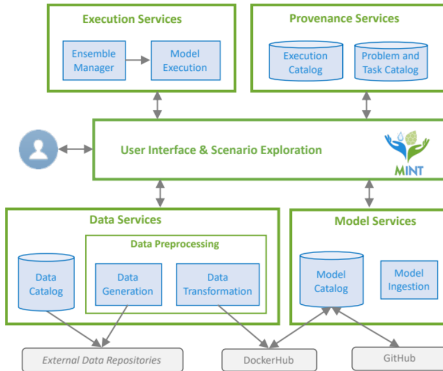
Figure 19: An overview of the MINT architecture, showing the interdependencies between its modules.
