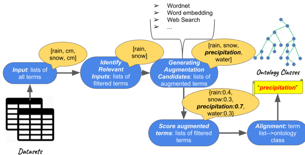
Figure 2: Generating additional keywords for datasets through a fuzzy augmentation process.
