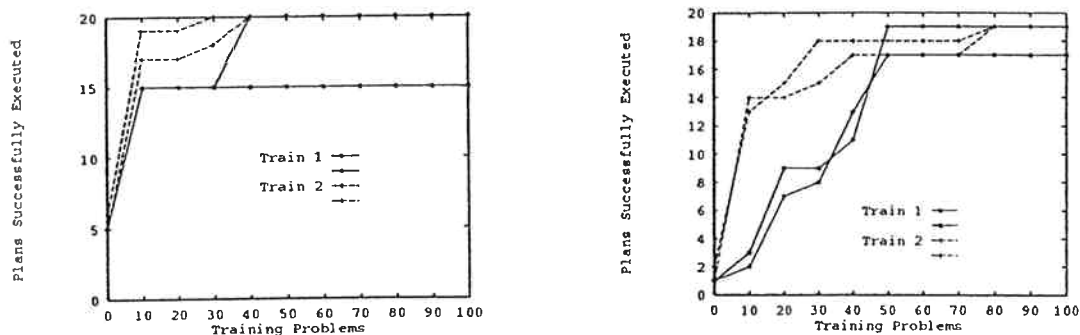
(b) Number of plans successfully executed in the test set
