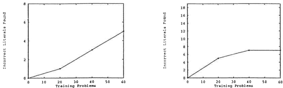
(a) Cumulative number of incorrect literals found during training
