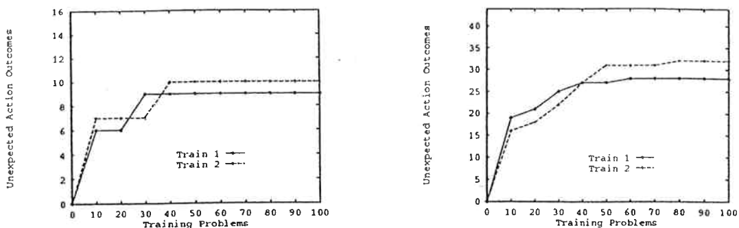
(a) Cumulative number of unexpected action outcomes during training
