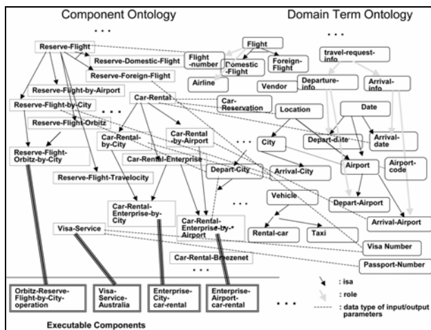
Figure 2. Example Component Ontology and Domain Term Ontology.
