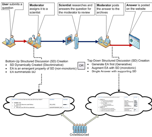
Figure 5: Structured Discussion (SD) formulation with respect to the Expert Answer (EA)
